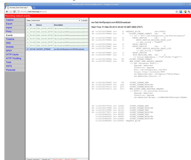
Figure 7. Socket internals page chrome://net-internals/#sockets
